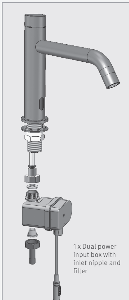
1 X FAUCET AND ATTACHMENTS
